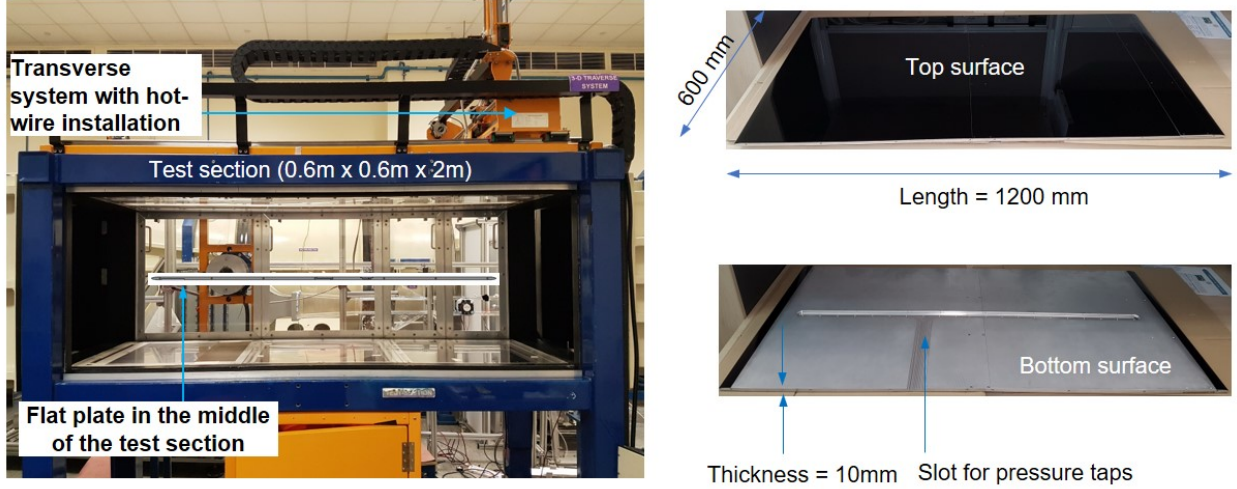
Fig. 4 Left: test-section of low-speed closed-loop wind tunnel used for experiments, with the flat plate installed. Right: Top and bottom surfaces of aluminum flat plate.
